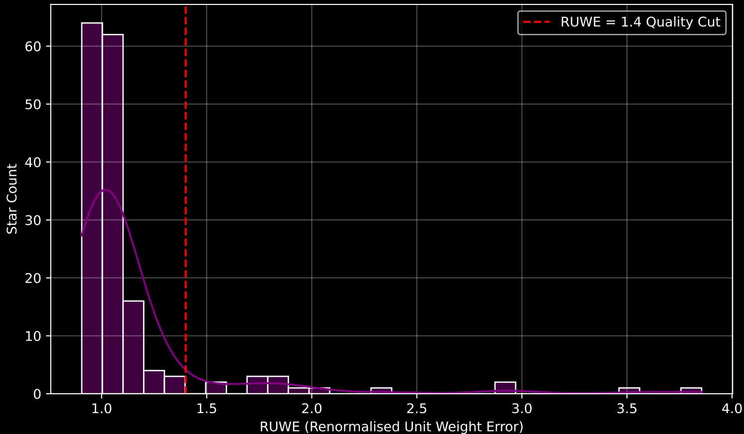
GAPOGEE DR17 Field [SA57-S] RUWE Distribution (n= 164)
