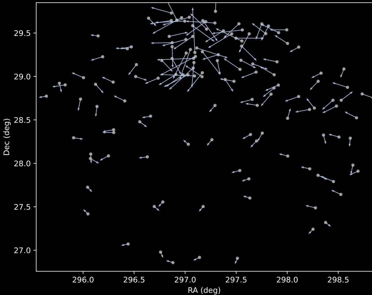
APOGEE DR17 Cluster 1 Proper Motion Vectors (n=135)
