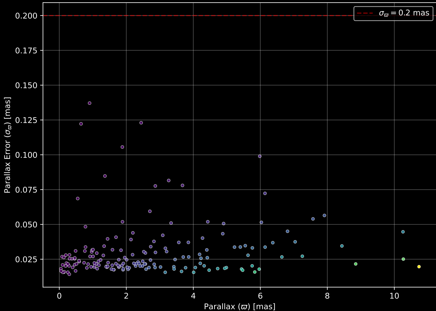
APOGEE DR17 Field: [SA57-S] Parallax Quality (n= 169)
