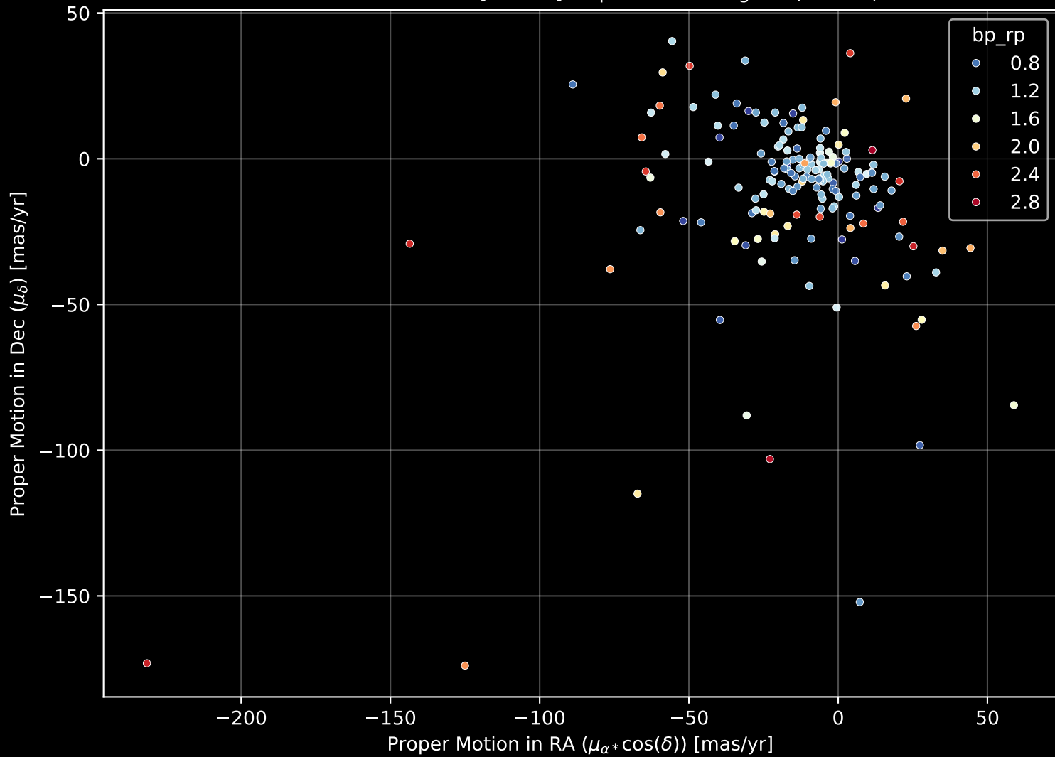
APOGEE DR17 Field: [SA57-S] Proper Motion Diagram (n= 169)
