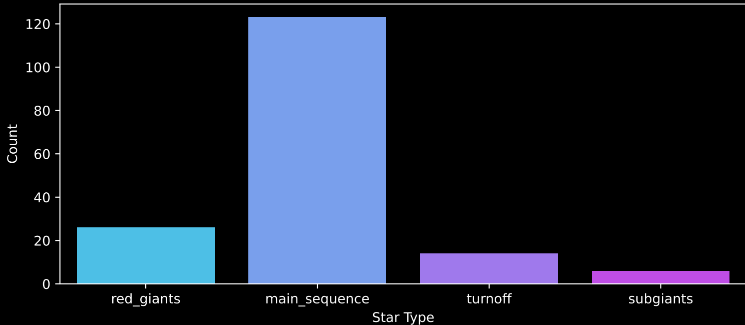
APOGEE DR17 Field: [SA57-S] Count plot of Star Type
