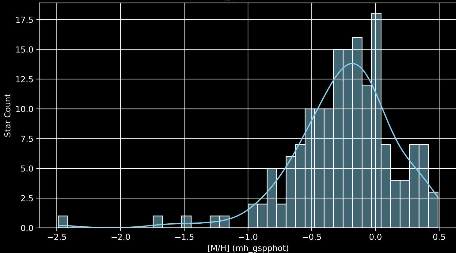
APOGEE DR17 Field: [SA57-S [M/H] (mh_gspphot) (n= 167)
